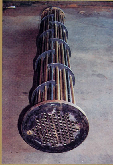
Intercooler and Aftercooler baffles are drilled to a tight tolerance hole for less vibration at baffle to tube contact.
