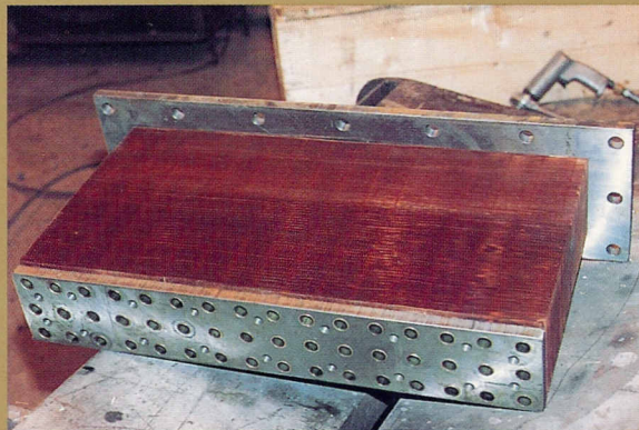
Replacement intercooler with Copper fins, Admiralty tubes and Carbon Steel tubesheets.
