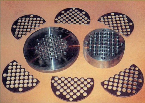
Tubesheets and Baffles. Tubesheets are made of Carbon Steel. Baffles are made of Mycrata and drilled to a tight hole tolerance to reduce wear on tubes.
