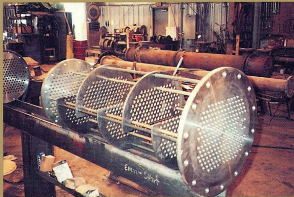
Intercooler skeleton, ready for tubing, 20" diameter x 50" long.
