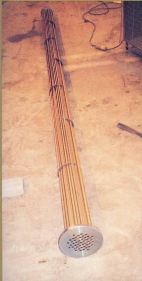
Aftercooler bundle, 6" x 12' with 1/2" O.D. Admiralty tubes, Brass tie rods and spacers. Front and rear tubesheet Carbon Steel.
