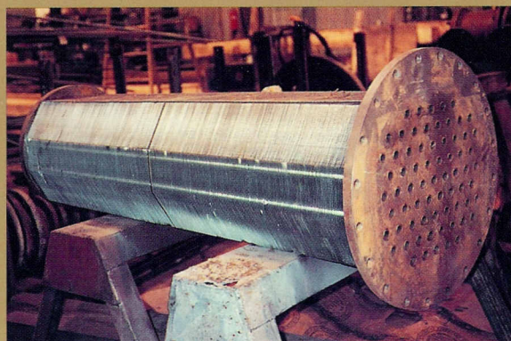
Intercooler bundle with Admiralty tubes, Carbon Steel tubesheets, and octagon-shaped Aluminum fins.
