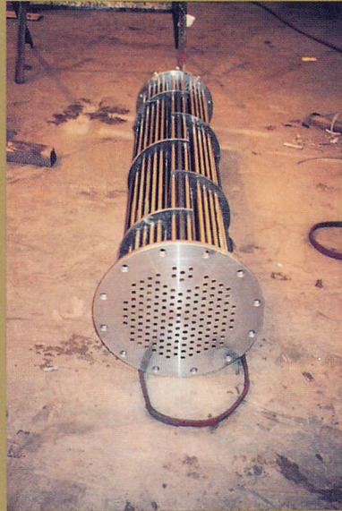
Intercooler, 18" x 74" with 5/8" O.D. Admiralty tubes, completed.
