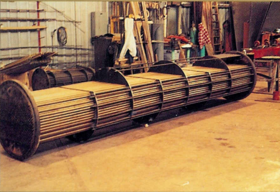
Large aftercooler with 710 pcs. 5/8" O.D. Admiralty tubes. Carbon Steel tubesheets were reused.
