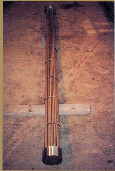
Aftercooler bundle, 6" x 9' with 3/8" O.D. Admiralty tubes. Brass tie rods and spacers are a standard on bundles. Stainless Steel skirt on the rear tubesheet strengthens the packing joint.
